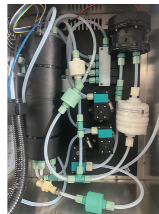
Ink system
